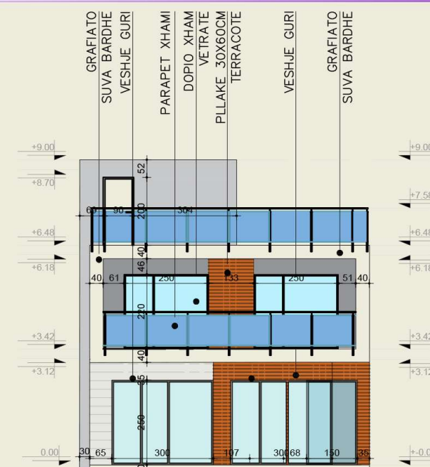
FASADE LINDORE SH:1:300
